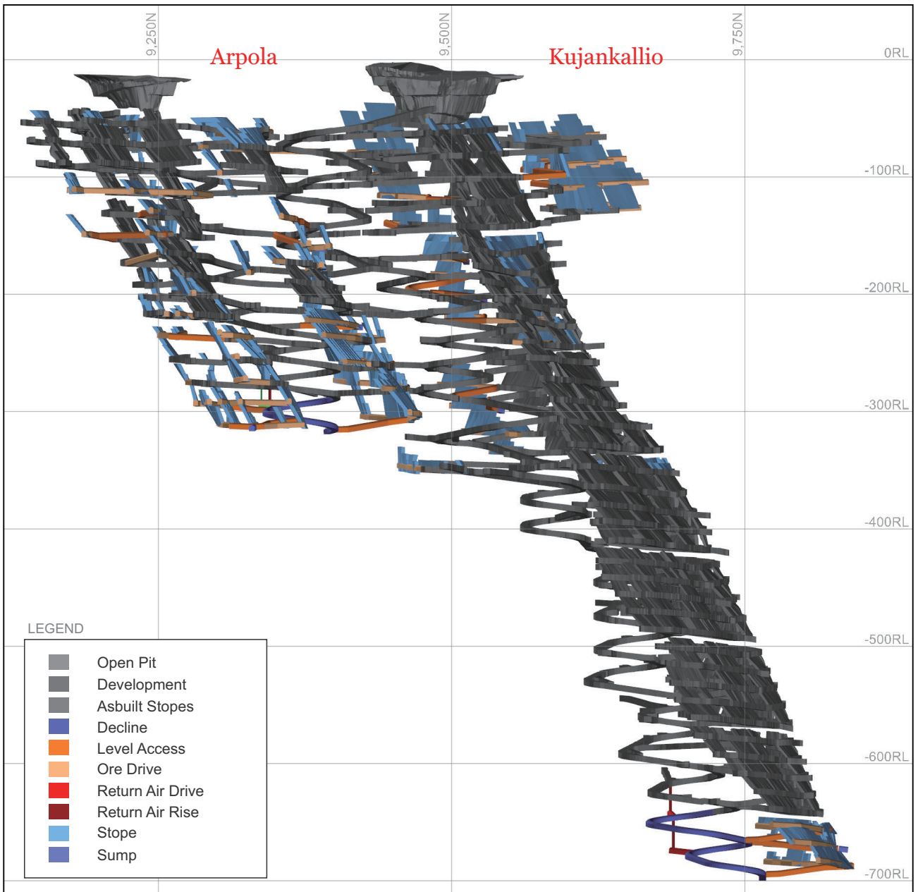
Figure 4 – Jokisivu Mine Design. Vertical View looking to the West.
