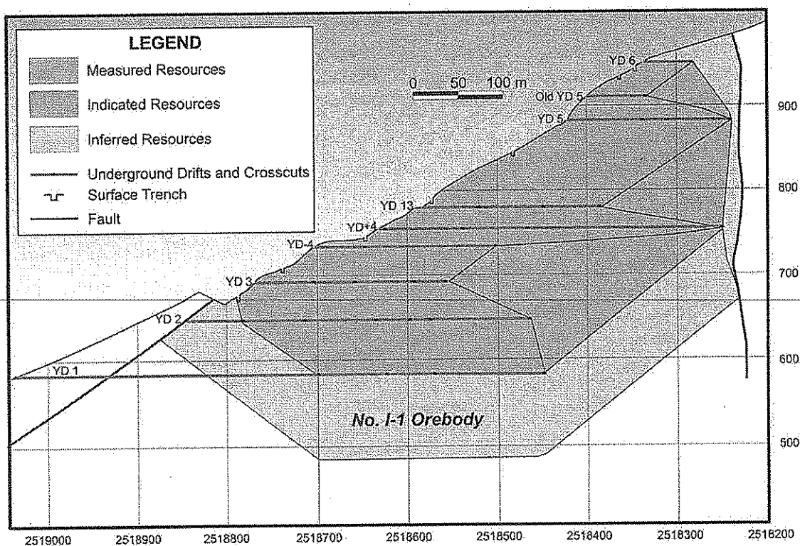
Figure 6.2 Block Mineral Resource Classification for the No.1-I Orebody
