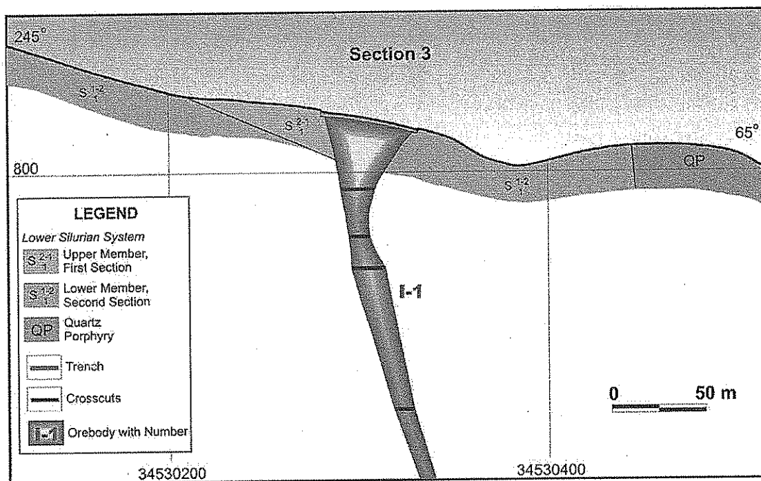
Figure 5.2 A typical Cross Section of the No. I-I Orebody in Damajianshan Deposit (Location of the section is shown in Figure 5.1.)
